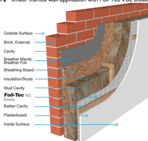
Diagram 2 - timber-framed wall application with Foil-Tec VCL Double
