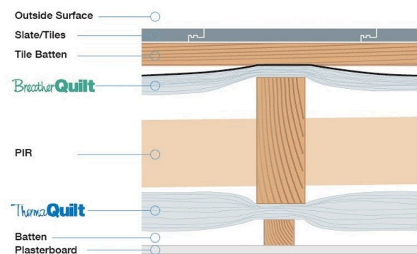
Diagram 2 - single layer - under rafters with BreatherQuilt
