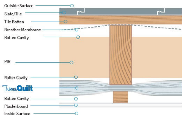
Diagram 1 - single layer - under rafters
