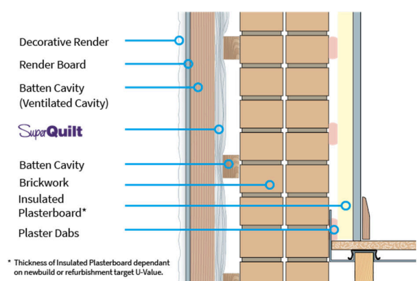
Diagram 4 - rendered external wall insulation
